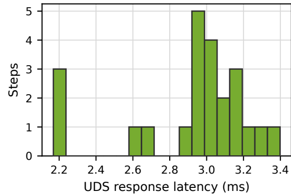
All lifecycle request latencies
