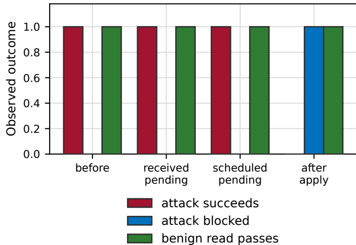
Lifecycle state behavior
